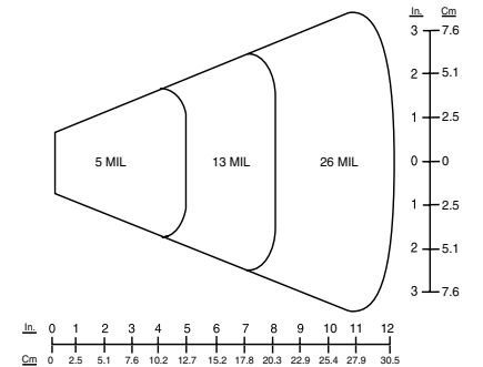
Typical reading zones on Code 39 bar codes
